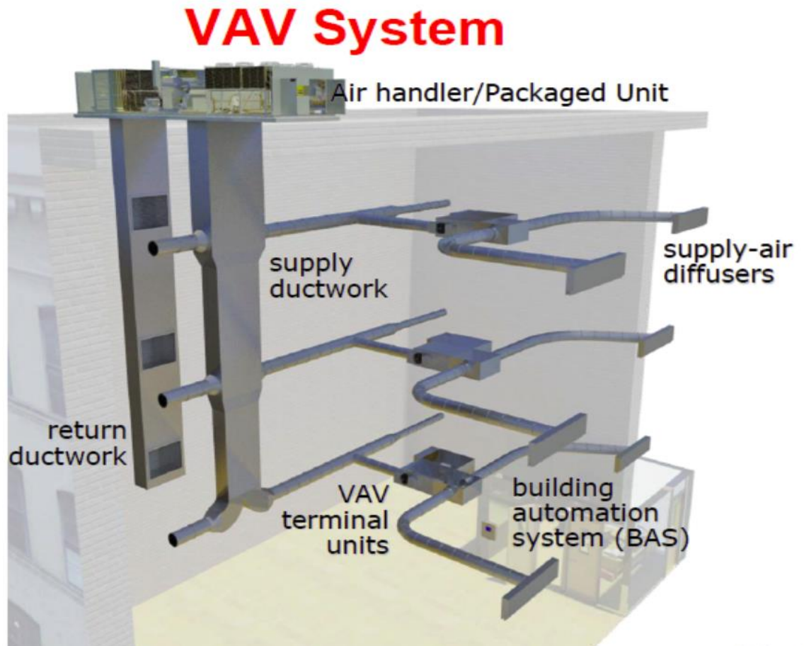
Figure 1 VAV system
